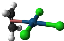
Zeise's salt, potassium trichloro(ethene)platinate (II) (the anion is shown) is the first organometallic complex containing a transition metal; prepared by Zeise in 1827. (Image from Wikipedia.)
