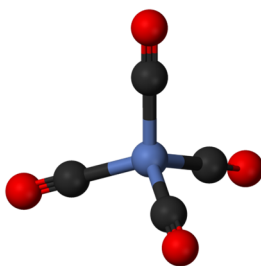
Tetracarbonylnickel(0), \text{Ni}(\text{CO})_4 , was discovered by Mond in 1890. It is one of the first "carbonyl" compounds and is a gas at room temperature. The Mond process is used to purify crude nickel ore. (Image from Wikipedia.)
