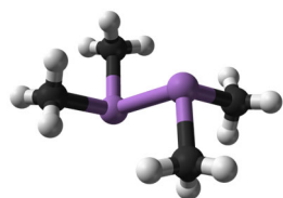
Cacodyl, also known as tetramethyldiarsine, is widely considered the first organometallic compound; prepared by Cadet de Gassicourt in 1757. (Image from Wikipedia.)
